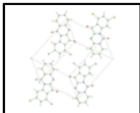
Fig. 2. Packing diagram for the title compound with displacement ellipsoids drawn at the 50% probability level. H atoms are omitted for clarity.
